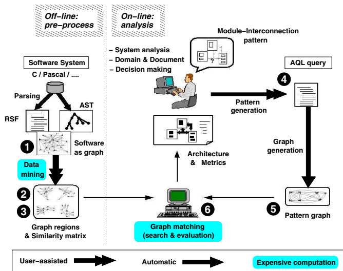
Figure 1. The proposed interactive environment for pattern-based software architecture recovery and evaluation.
